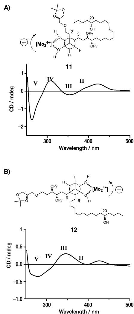
Figure 3. Circular dichroism curves of chiral \text{MO}_2 -dimer complexes of the isolated diol derivatives 11 (A) and 12 (B). Roman numbers indicate the diagnostic CE bands following Sznatzke and Frelek's nomenclature.
