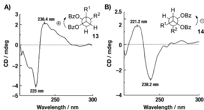
Figure 4. Circular dichroism curves of dibenzoyl derivatives 13 (A) and 14 (B). The inserts show the suggested chiralities of the two dibenzoates in agreement with Harada and Nakanishi model. [9] A, B) R 1 = glycerol-containing part. A) R 2 = C 5 –C 24 alkyl chain. B) R 2 = C 9 –C 24 alkyl chain.
