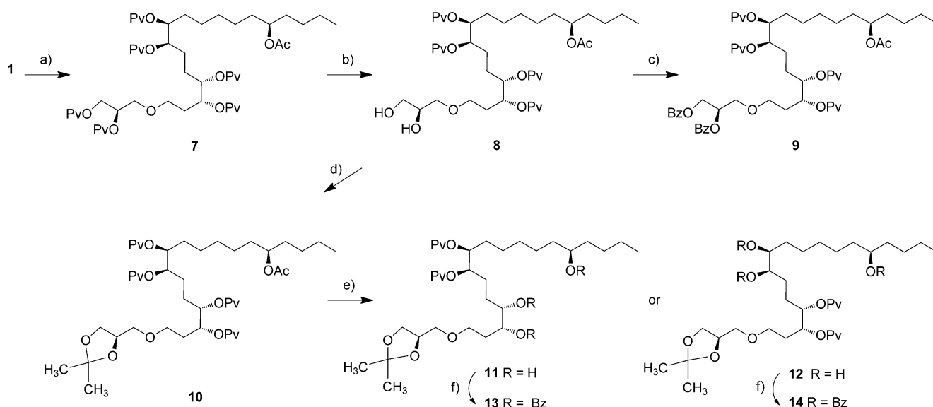
Scheme 1. Selective derivatization of mycalol ( 1 ). a) PvCl , dry pyridine, RT; b) Na_2CO_3 , MeOH RT, overnight; c) BzCl (4 equiv), dry pyridine, RT overnight; d) (CH_3)_2C(OCH_3)_2 , PPTS, 75 °C, 6 h; e) Na_2CO_3 , MeOH RT, 72 h, chromatographic resolution; f) excess BzCl , dry pyridine, 50 °C, 24 h. Bz = benzoyl, Pv = pivaloyl.
